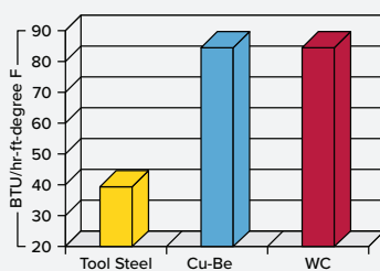
Thermal Conductivity
